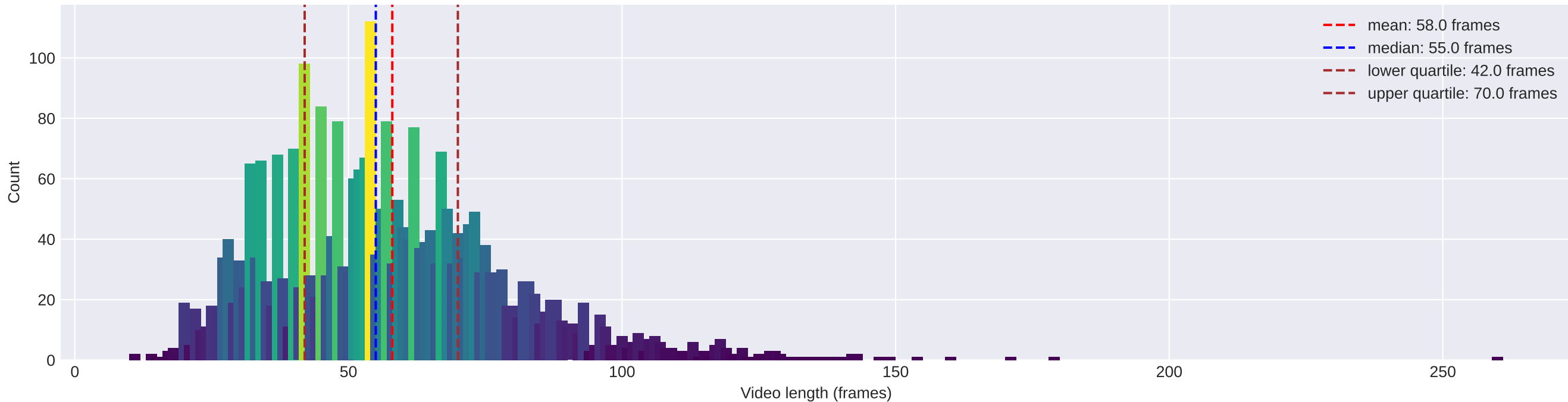
Video length Distribution: asl2000 / test
